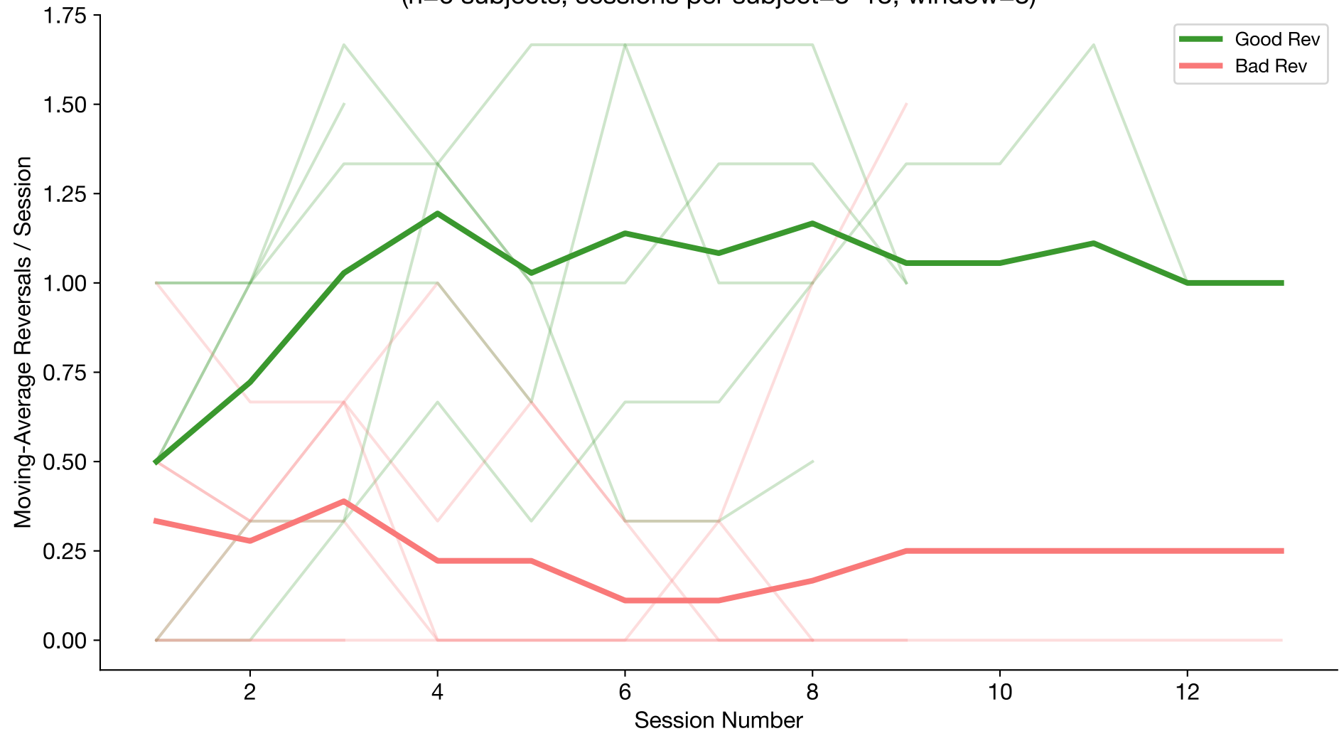
Moving-Average Good and Bad Reversals Over Time (n=6 subjects; sessions per subject=3–13; window=3)
